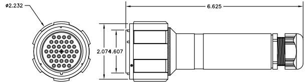
TL-37-LF06: 37 PIN FEMALE CABLE MOUNT CONNECTOR
