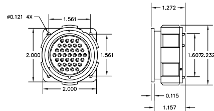
TL-37-PF26: 37 PIN FEMALE PANEL MOUNT CONNECTOR
