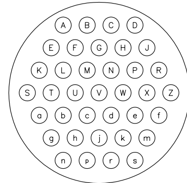
TL-37-PF26: 37 PIN FEMALE CONNECTOR
