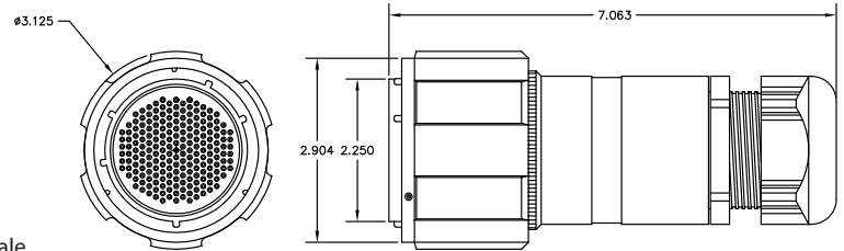
TL-201-LF06: 201 PIN FEMALE CABLE MOUNT CONNECTOR
