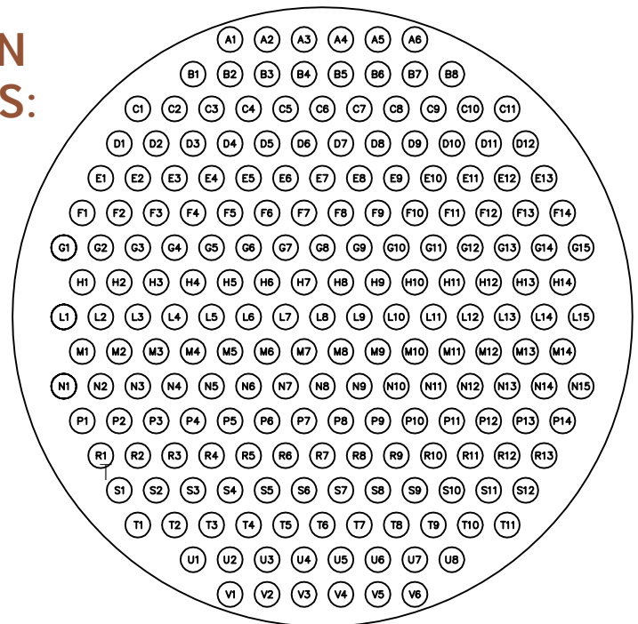
TL-201-PM26: 201 PIN FEMALE CONNECTOR
