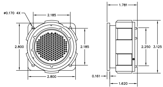
TL-201-PM26: 201 PIN FEMALE PANEL MOUNT CONNECTOR
