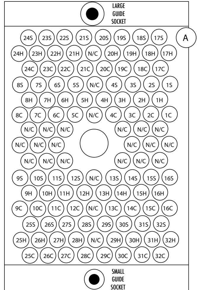
REAR VIEW
